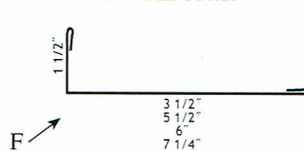
Ⓘ Post Trim 10'2" TLPT10xx
