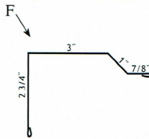
Ⓑ Residential Rake 10'2" TLRR18xx
