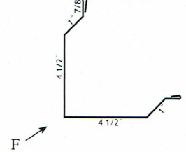
Ⓓ Rake and Corner 10'2" TLRC2xx
