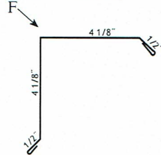
Ⓕ AG 4 Gable Trim 10'2" TLAG4xx
