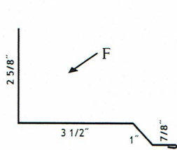
Ⓔ Univ. Sidewall 10'2" TLUS8xx
