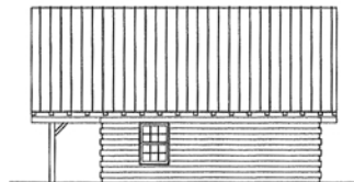
RIGHT SIDE ELEVATION
