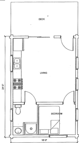
FLOOR PLAN
